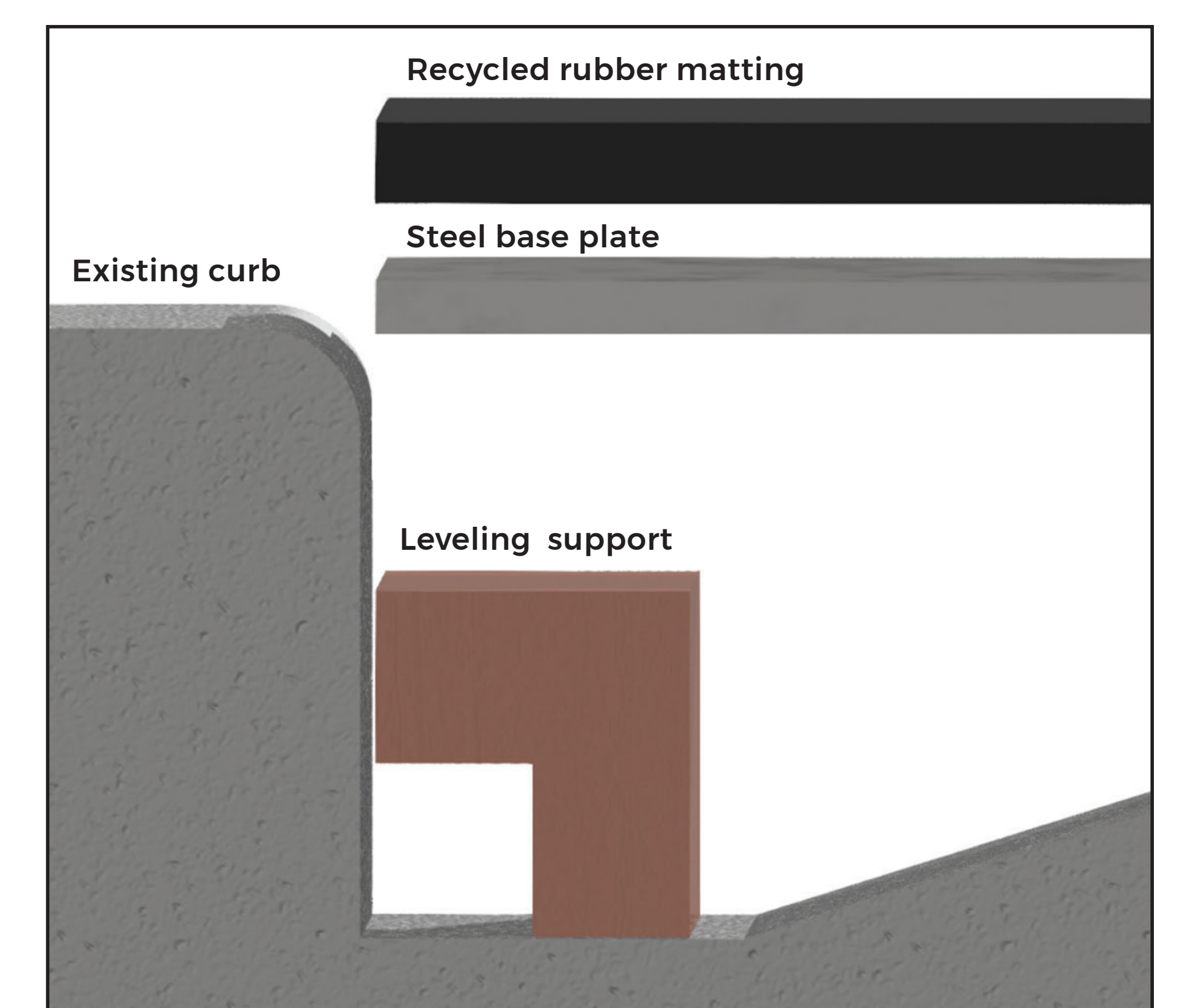
BASE - CURB DETAIL
